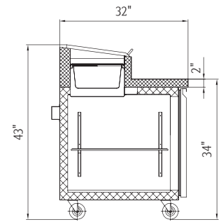
Side Section
